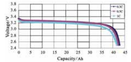
Discharge Curve in Normal Temperature
