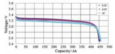
Discharge Curve in Normal Temperature
