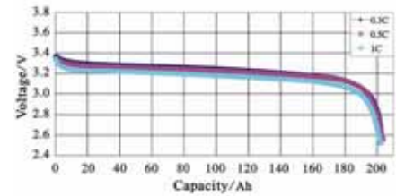
Discharge Curve in Normal Temperature
